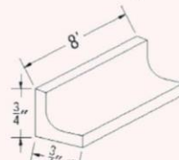
Inside Corner Molding
