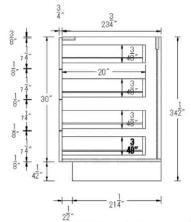
Kitchen 4 Drawers Base Standard
