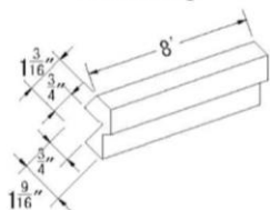
Cabinet Angle Molding
